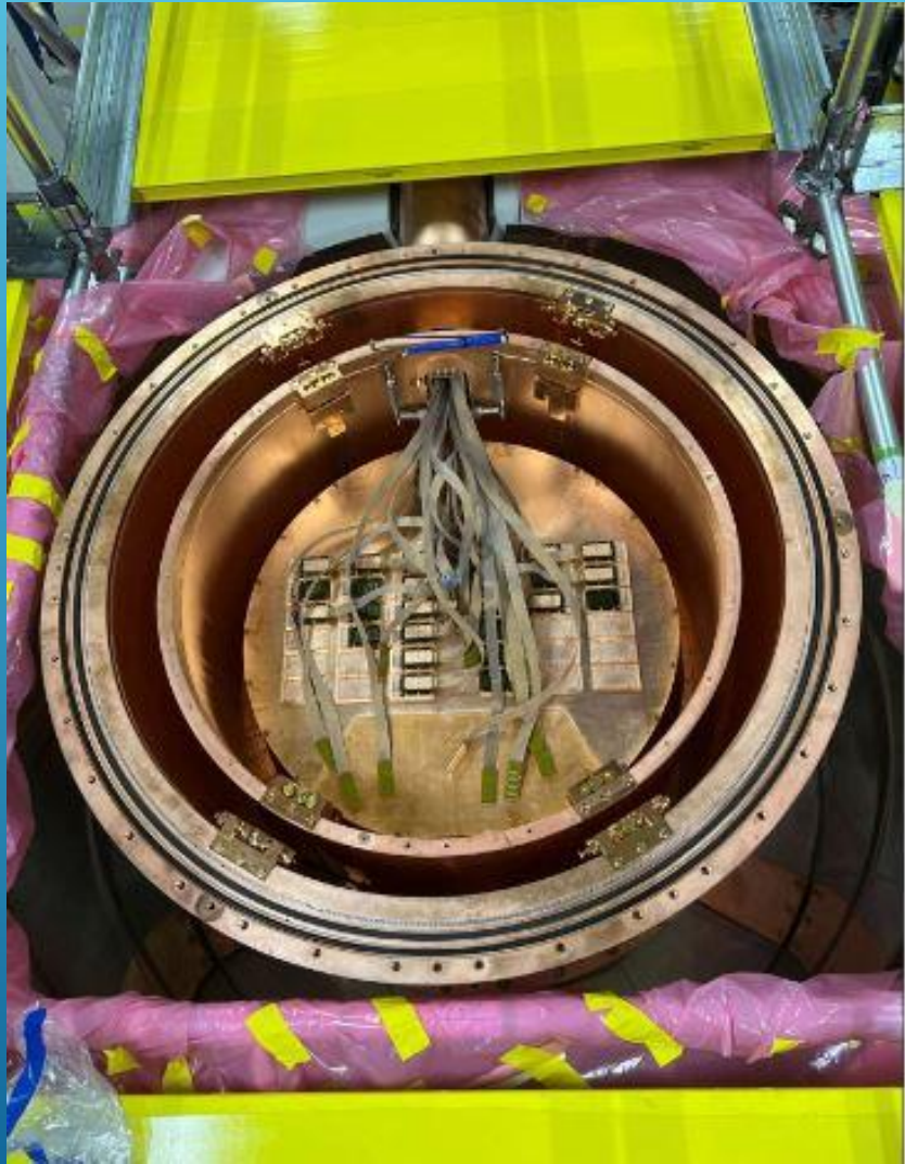
Detector Readout Cables connection
