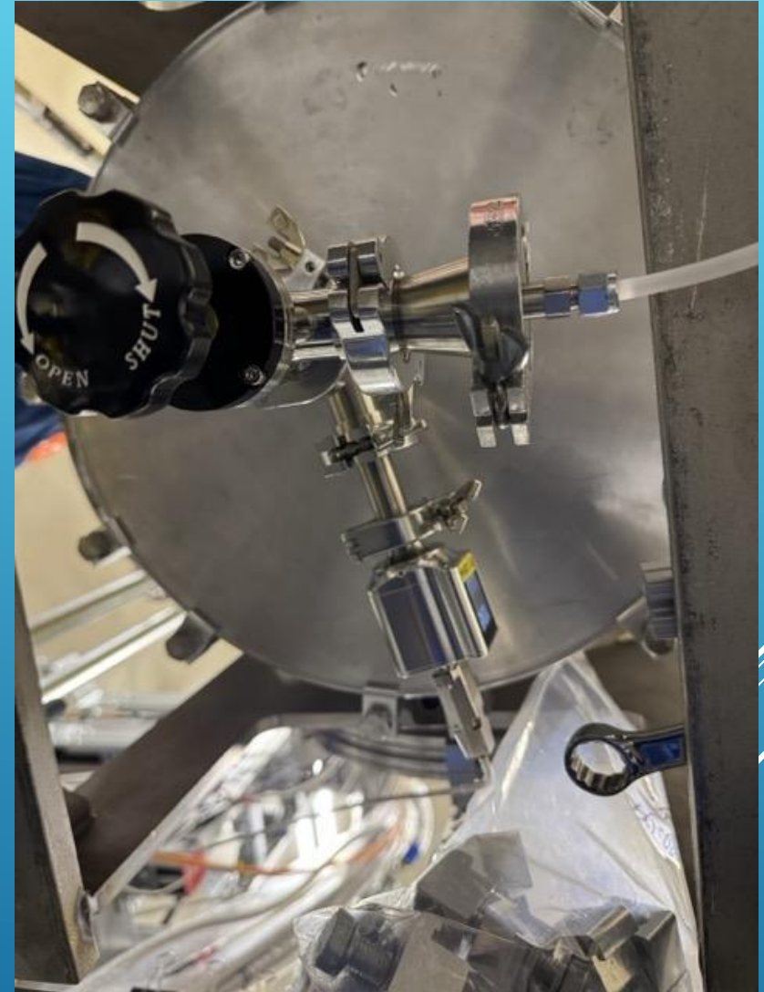
Cryostat purge
