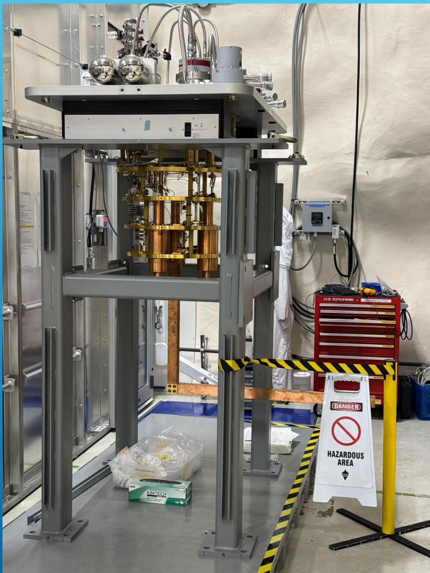
Dilution fridge on temporary stand
