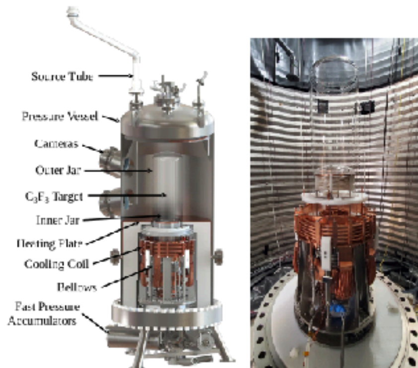
Figure 1. (Left) Schematic side-view of the PICO-40L pressure vessel with the major detector components labelled. The outer synthetic fused silica vessel houses the C 3 F 8 target. Two of the four camera ports are visible on the left of the pressure vessel. The heating plate and cooling coil maintain the temperatures of the two thermal zones. The fast accumulators allow for rapid recompression of the chamber after a bubble is formed. The calibration (source) tube can be seen penetrating the pressure vessel on the left. (Right) The PICO-40L inner assembly assembled inside the water tank.
