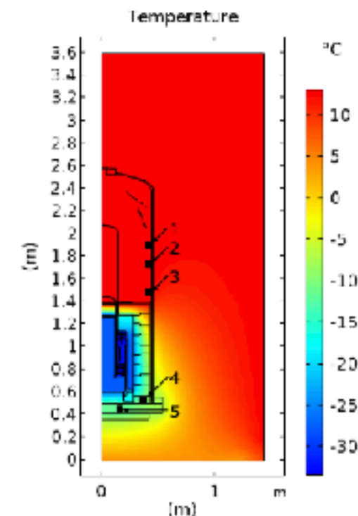
Figure 7. Temperature profile of a 2-dimensional axisymmetric simulation of a simplified model of the PICO-40L detector, after reaching equilibrium. The numbered black squares correspond to locations of RTDs in the detector, and a comparison to commissioning data is shown in Table 1. All simulated temperatures are within a few of the measured temperatures.
